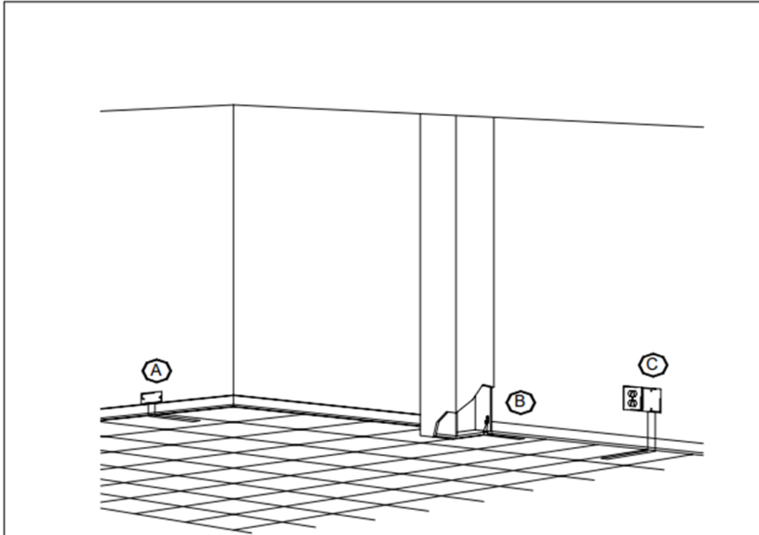
Common accepted ESD Tile system grounding methods
